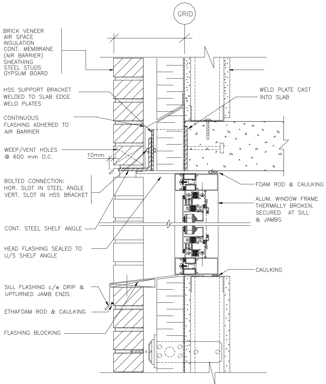
Detail 4.6 – Alternate Brick Veneer / Steel Stud Window Head and Sill Detail
