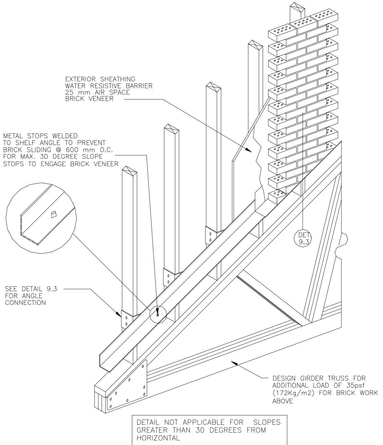
Detail 9.2 – Brick Veneer Supported by Truss (Typical Over Attached Garages)
