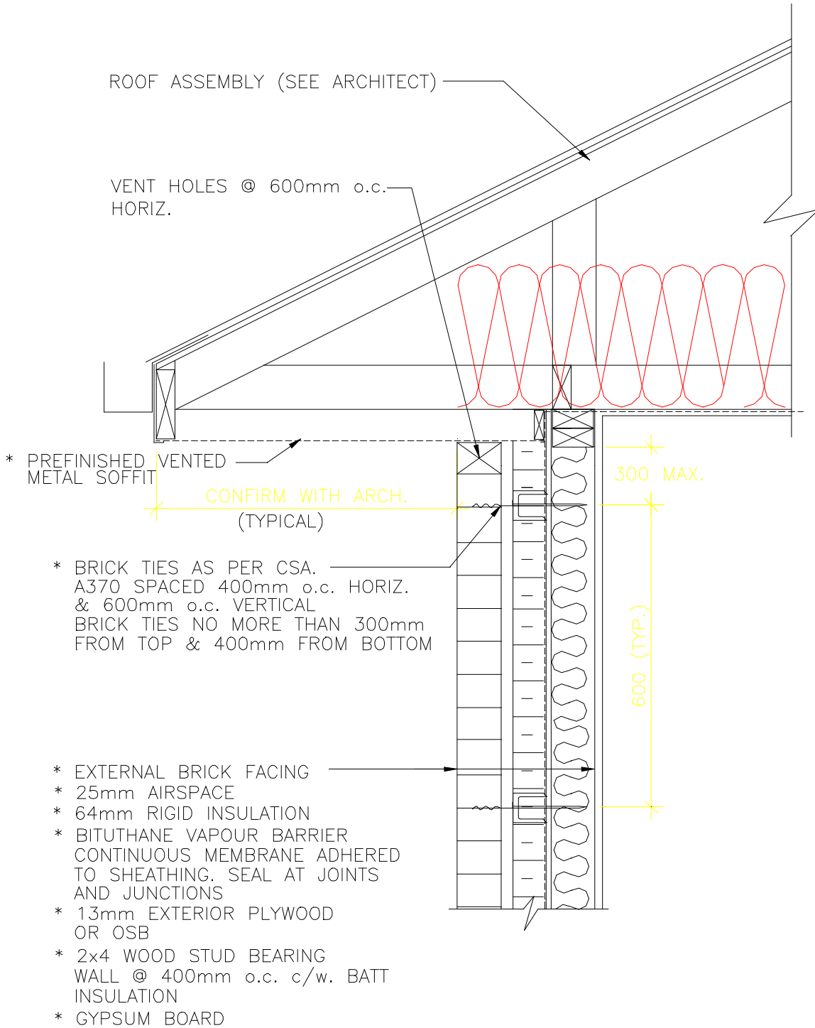
Detail 9.20 – Roof Truss Bearing on Load Bearing Stud Wall
